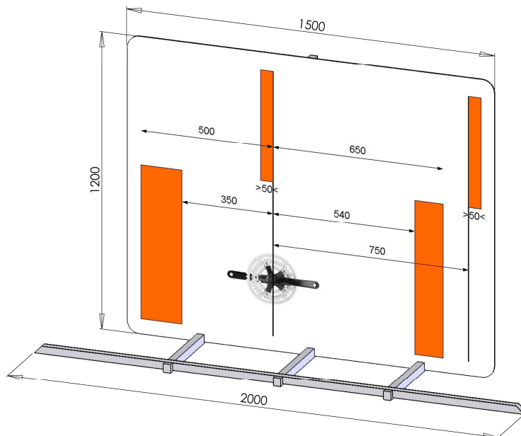
Figure 2: Example of a panel mounted on a measuring jig with a guide rail
